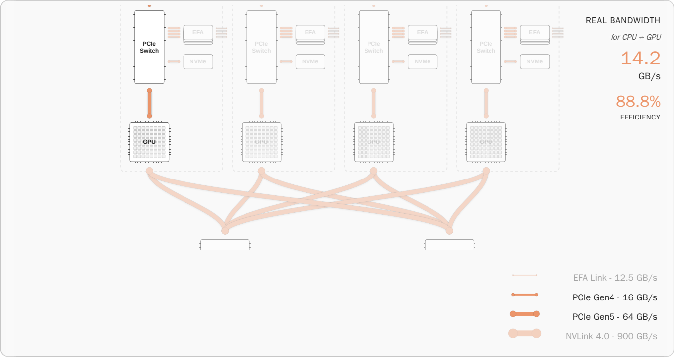
Figure 15 · Interactive diagram of key components and communication links in an AWS p5 instance. Shows the different GPU-GPU communication paths with their actual bandwidths.
