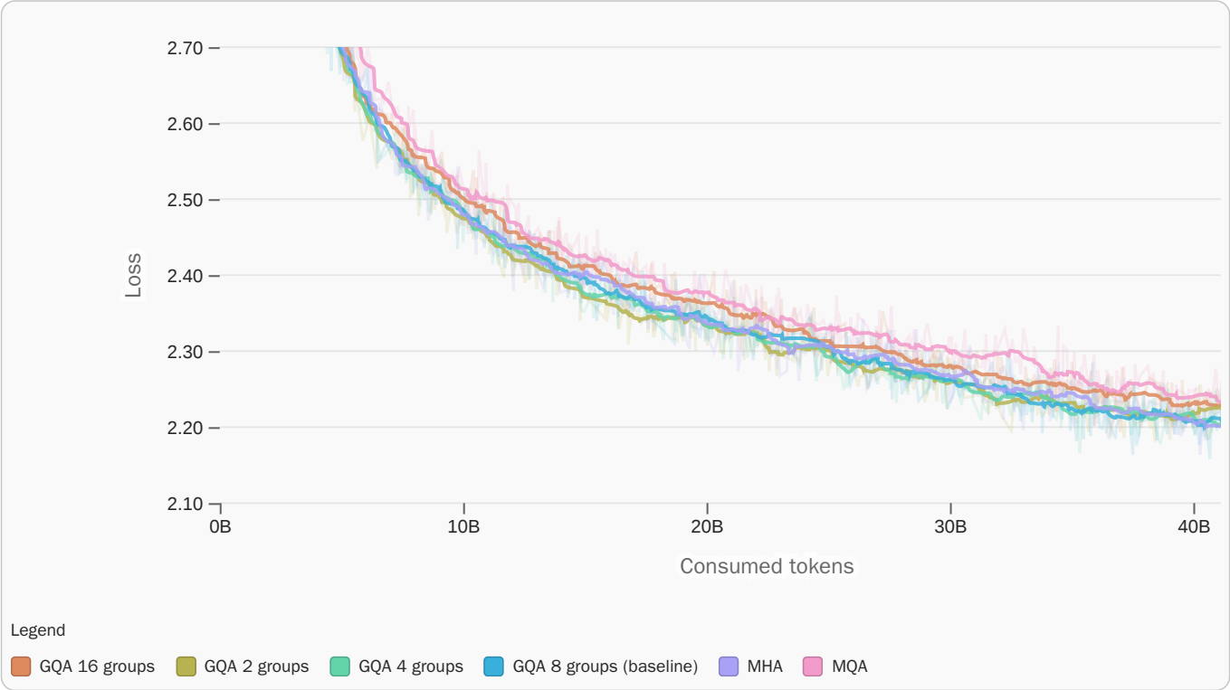
Figure 18 · Configurable line chart with zoom/pan, smoothing and interactive tooltips. Example with loss data for different attention configurations. Credit: SmolLM Training Playbook
