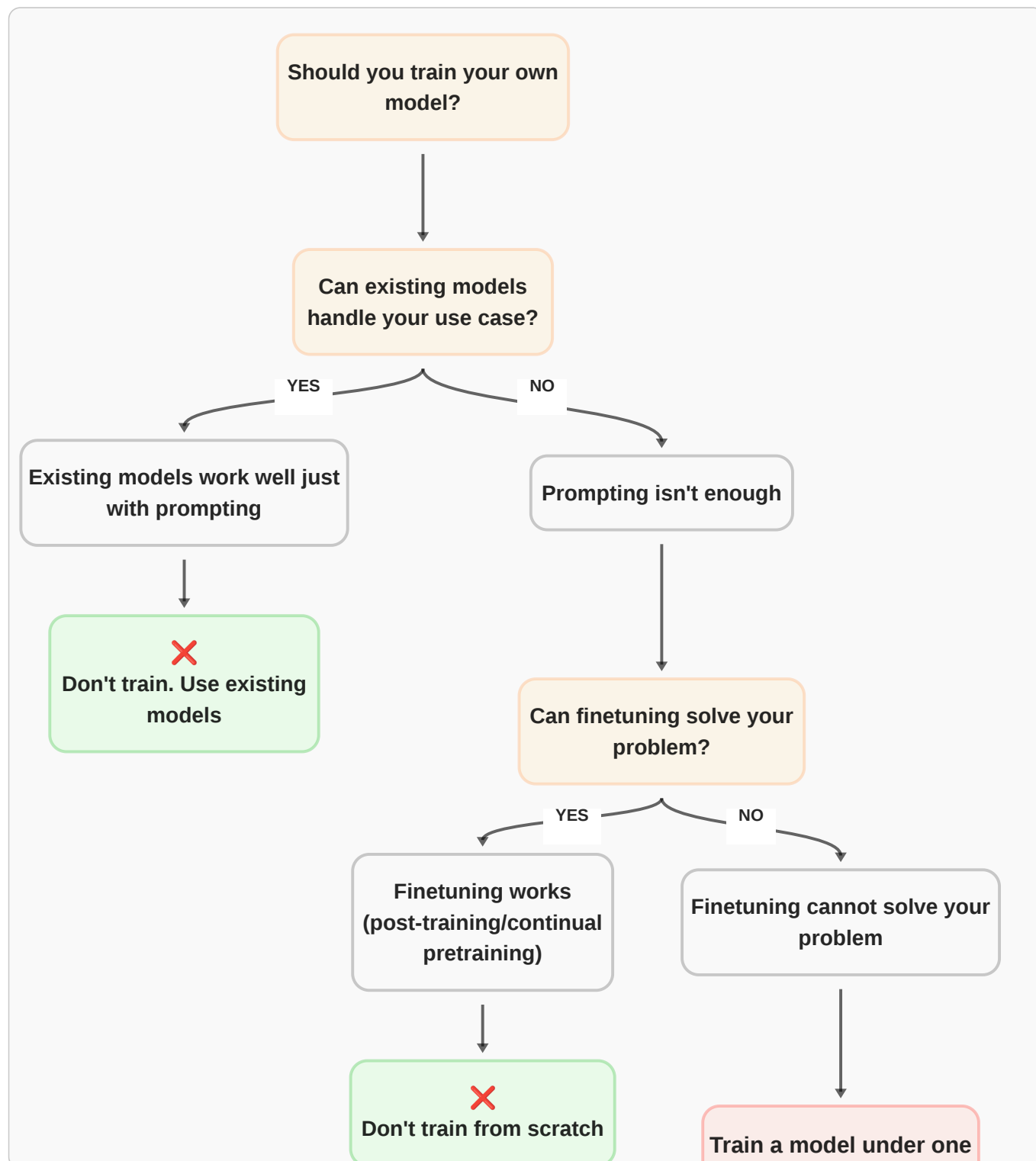
Figure 17 · Interactive decision tree to determine whether you should train your own model. Guides the thought process through key questions: Can existing models handle your use case? Should you fine-tune or train from scratch? For research, production, or strategic open-source?
